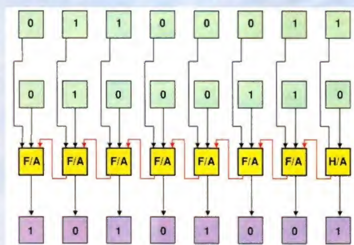
And this is how you combine the two to create a complete logic circuit for adding an eight-digit binary number. Don't worry if you don't understand this (I don't!) so long as you can follow how the two above get the right results.
